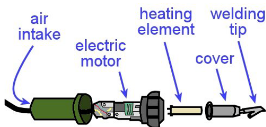
Heat welder
